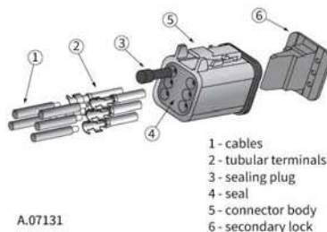
Connector plug (option) Deutsch DT 6-pin
